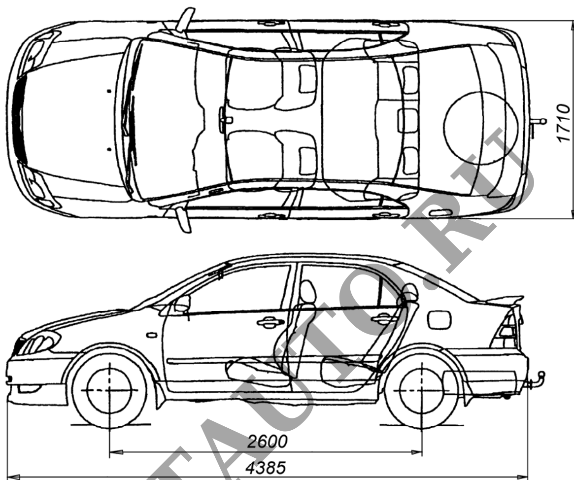
Toyota Corolla 4-door sedan
