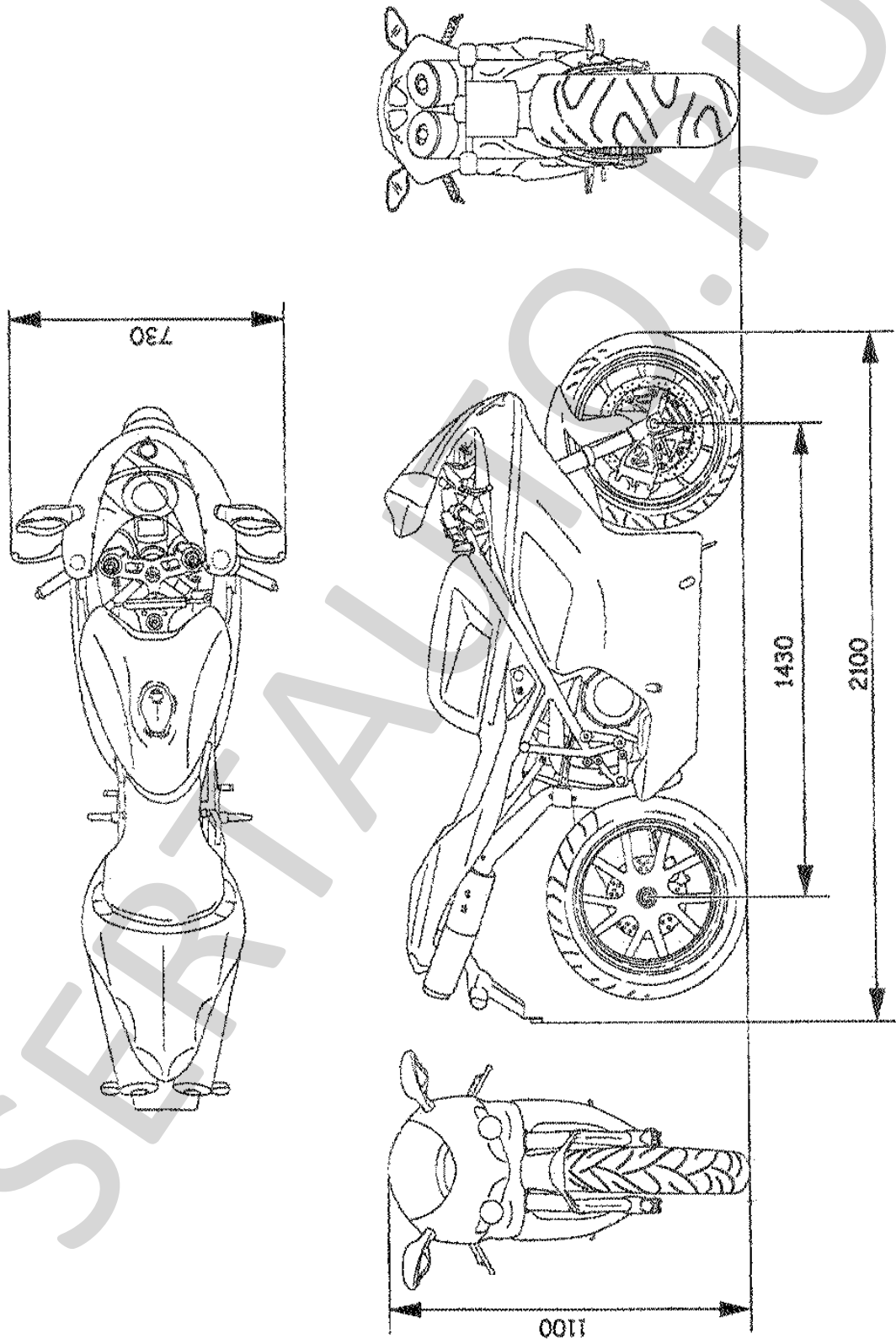
Рис. 1. Мотоцикл DUCATI H7 (1098, 1098S, 1098S Tricolore, 1098R, 1098R monoposto, 1098R biposto - SUPERBIKE )
